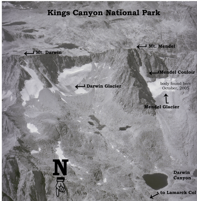
Aerial view of Darwin and Mendel Glaciers which allows visualization of topography
